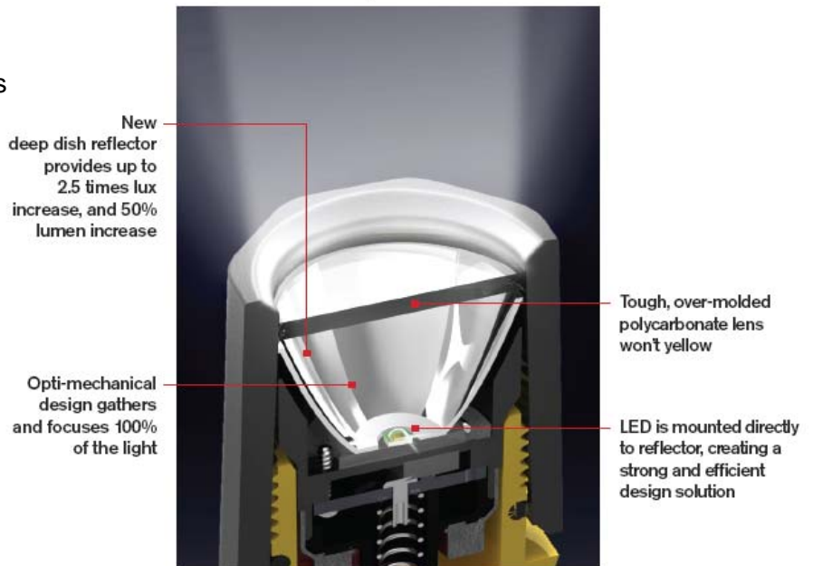
Flashlight section view
