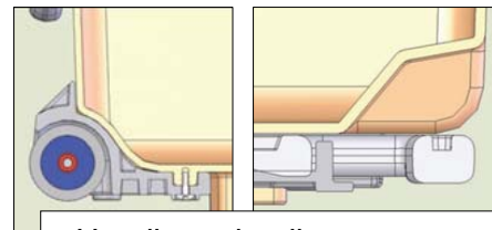
Handle and trolley recess areas deepened to accept the 1640 Transport Case dolly and wheels.
